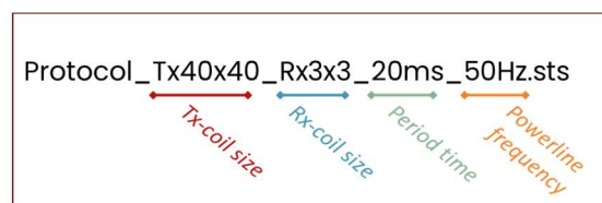
Figure 13. Protocol naming.
