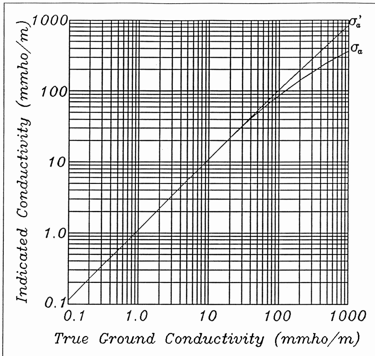
Figure 2: Conductivity Correction: Instrument on the ground surface
