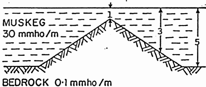
Fig. 5 CROSS SECTION BURIED RIVER VALLEY
